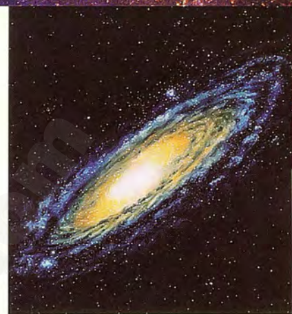
a depiction of our Milky Way
